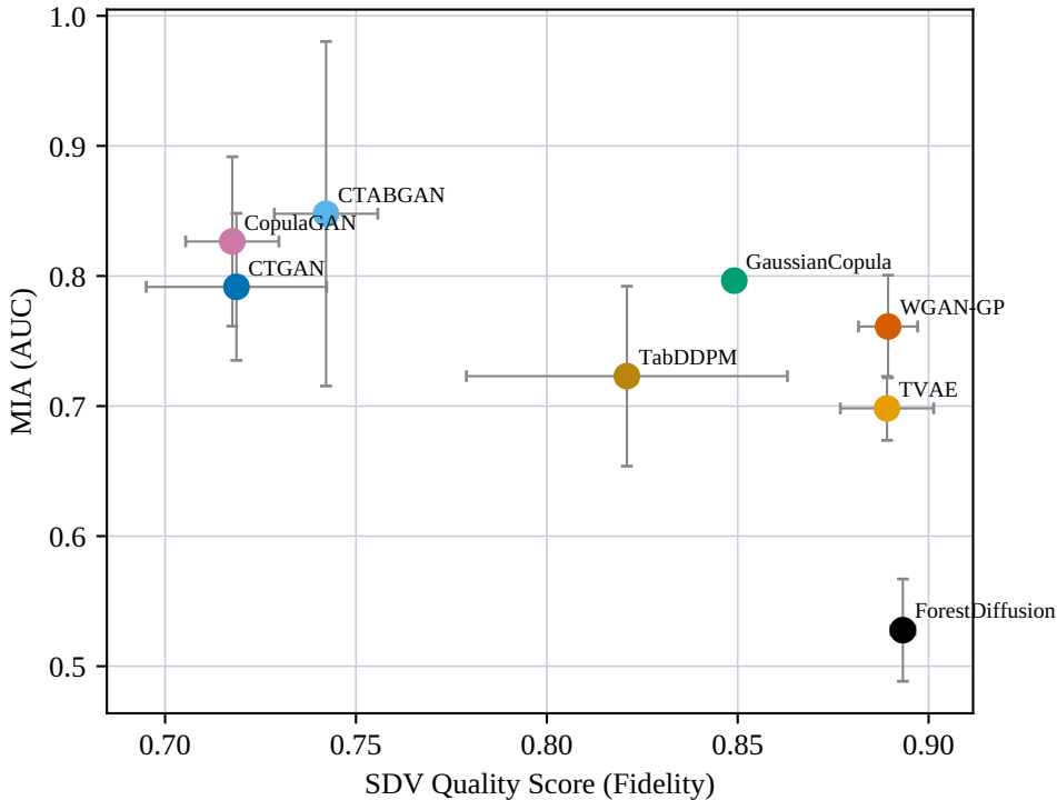
Concrete: SDV Quality Score (Fidelity) vs MIA (AUC)
